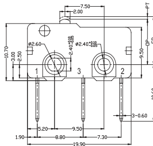
Quick Connect Terminals (Thickness: 0.6 mm)
