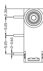
L Left Angled PCB Terminals
