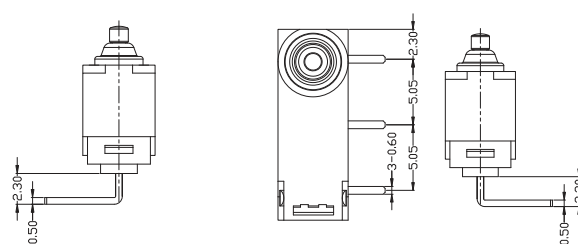
R Right Angled PCB Terminals
