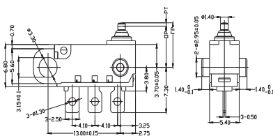
7 M3 type post
