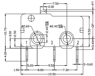
Straight PCB Terminals
