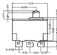
19 27 D1/D2 type two side posts
